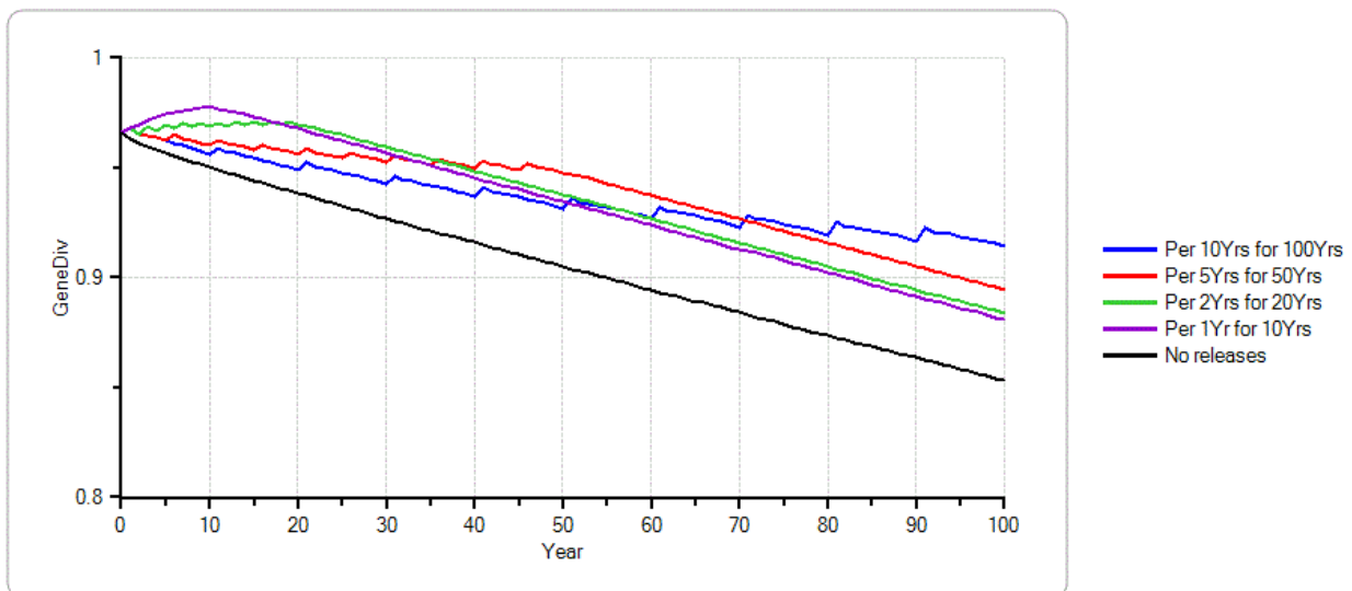
Figure 7. Projected loss in GD in NL VIM population under favorable conditions under different supplementation schedules (100 VIMs released per scenario) and with no supplementation (black line).
