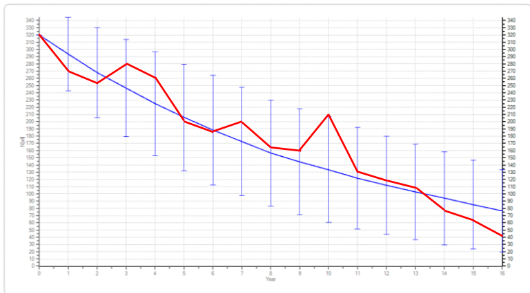
Figure 4. Retrospective model projection (in blue) of VIM meta-population from 1984 to 2000 (bars indicate SD). Mean census counts shown in red.
