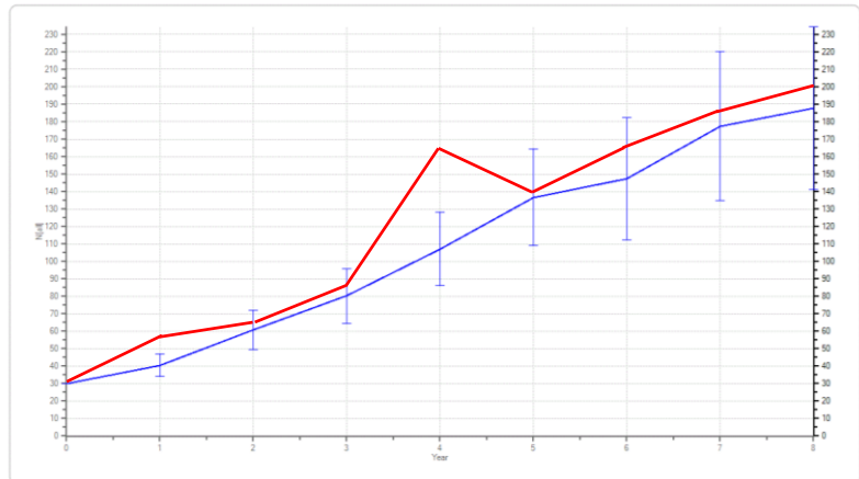
Figure 3. Retrospective model projection (in blue) of NL VIM population from 2005 to 2013 (bars indicate SD). Mean census counts shown in red.
