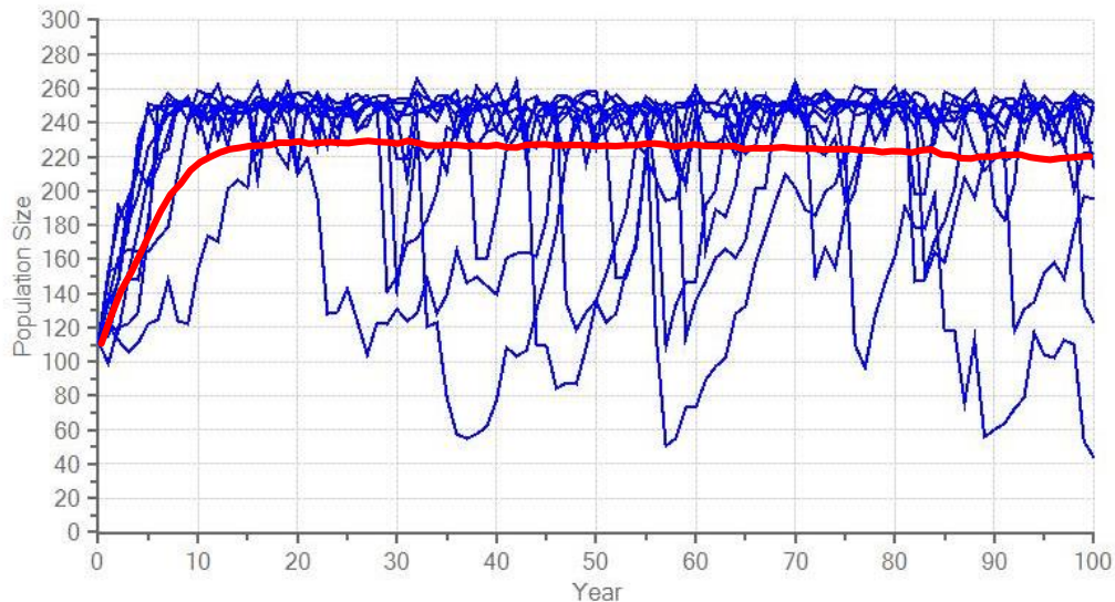
Figure 5. Example projection of population size over time for 10 iterations (blue lines). Mean population size for 1000 iterations is indicated by the red line.
