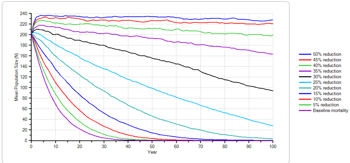
Figure 10. Projected mean population size for VIM populations under high mortality conditions (baseline) and with various levels of mortality reduction.
