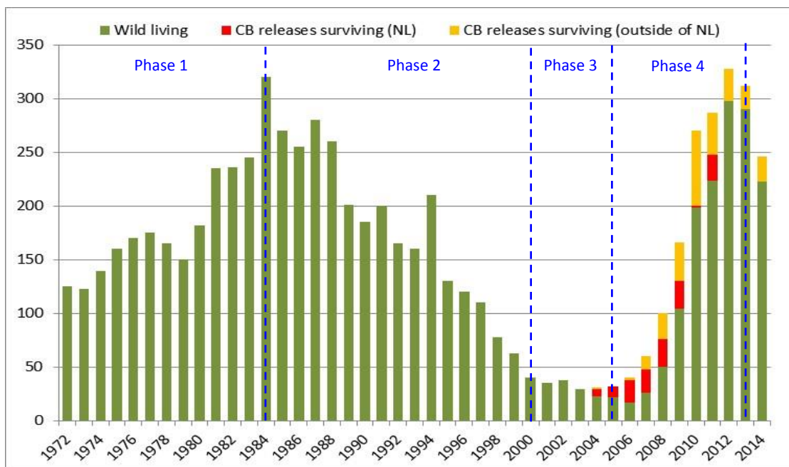
Figure 1. Total meta-population estimates for wild Vancouver Island marmots from 1972 to 2014. Red and yellow bar portions represent marmots released in that year and that survived to fall counts. Phases indicate different population trends specified for modeling purposes.
