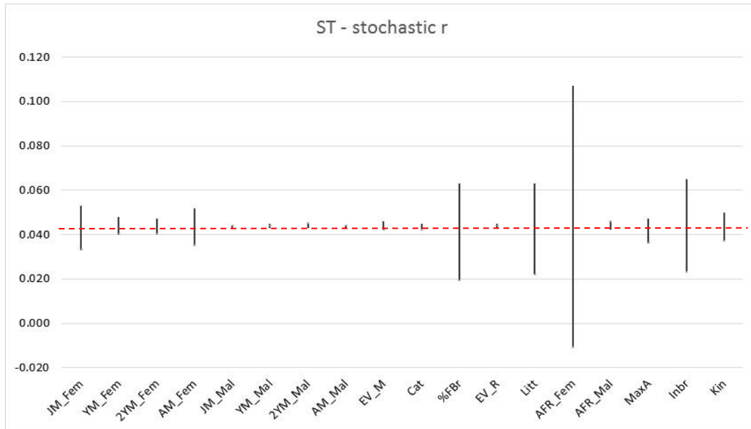
Figure 2. Stochastic r for input values tested in sensitivity analysis. High and low values are indicated by the line for each parameter; red dashed line indicates base model values. Parameters follow the order in the list above.
