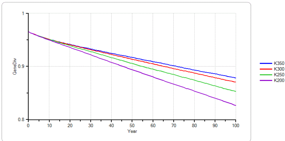
Figure 6. Projected loss in GD in NL VIM population under favorable conditions under different carrying capacity values.
